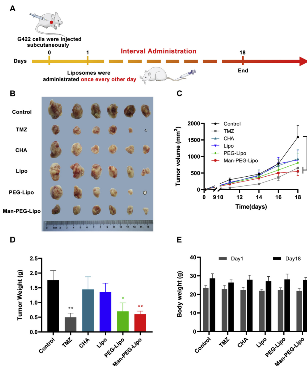
Fig. 7. In vivo antitumor efficacy and safety evaluation of CHA-encapsulated liposomes using interval administration. (A) The schematic of treatment schedule. The images of excised tumors (B), tumor volume changes (C), tumor weight (D), and body weight changes (E) of murine G422 glioma tumor-bearing mice after interval intravenous treatment of CHA-encapsulated liposomes. Each value represents the mean \pm SEM (n = 6). *p < 0.05, **p < 0.01, and ***p < 0.001 compared with the control group.
